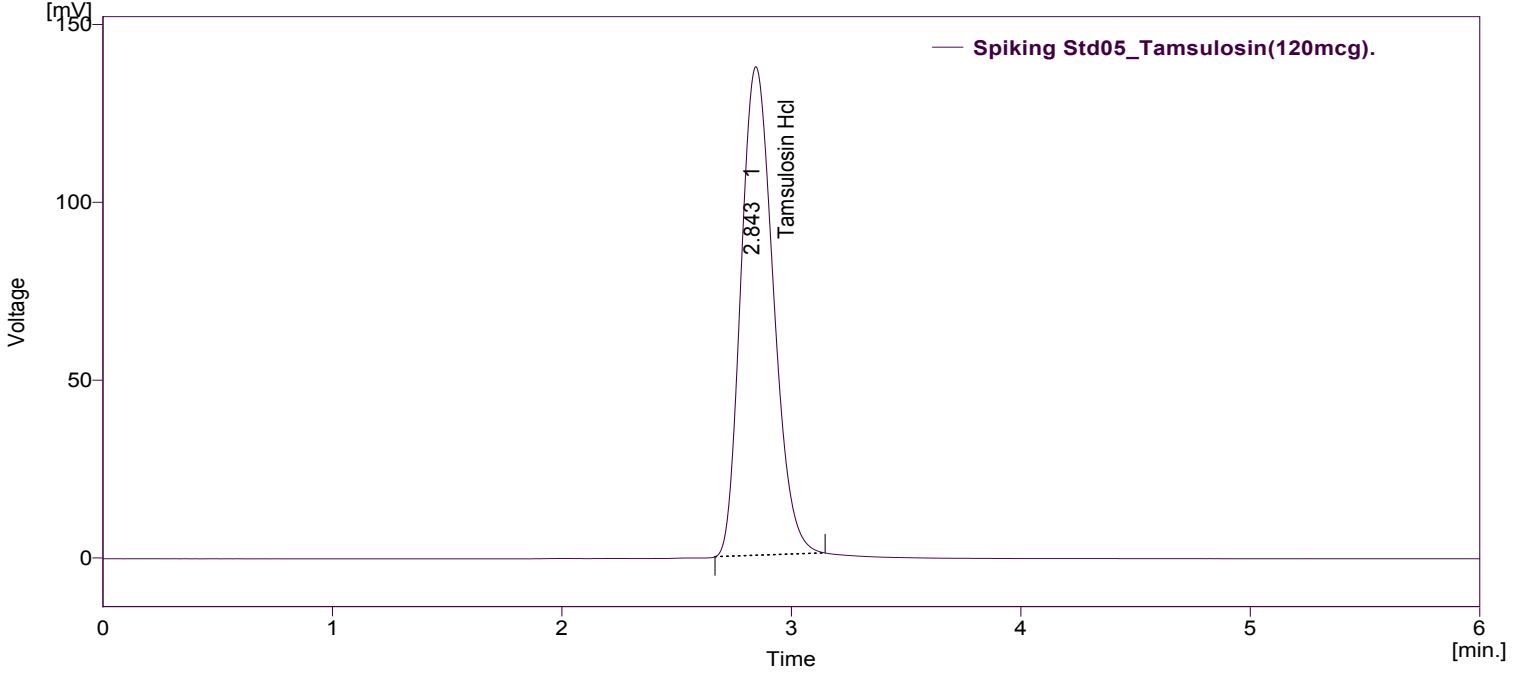
Result Table (Uncal - Spiking Std05_Tamsulosin(120mcg).)
